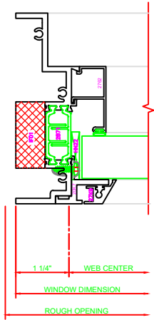
403 JAMB SERIES: 450G FIXED
