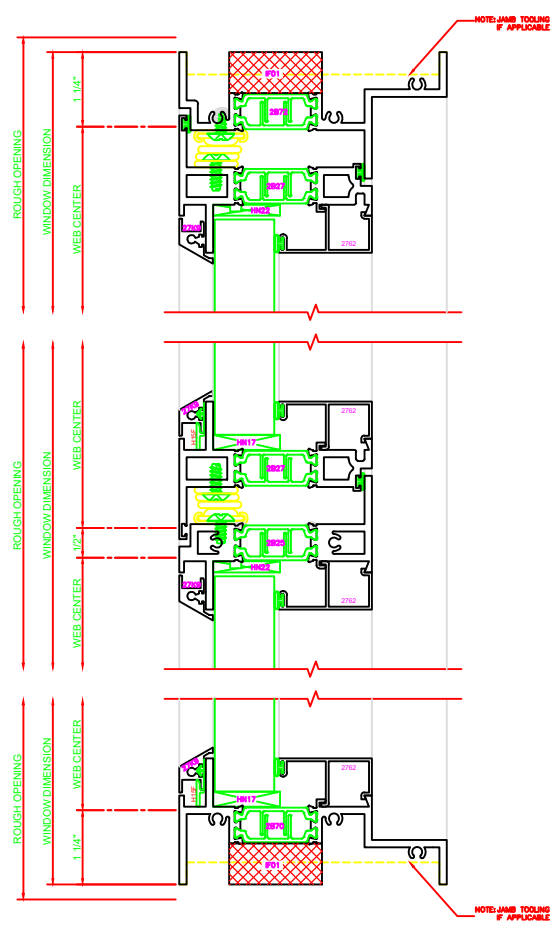
542 MEETING RAIL SERIES: 450G C.O./FIXED 4-BAR ARMS
