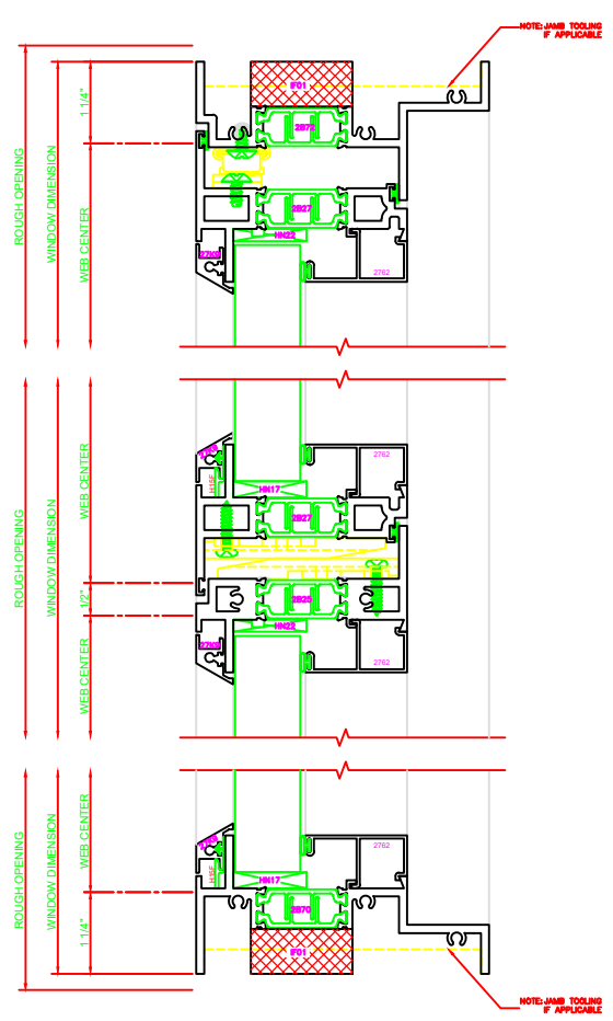
543 MEETING RAIL SERIES: 450G C.O./FIXED BUTT HINGE
