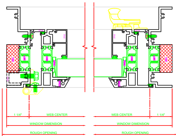
445 JAMB SERIES: 450G CASEMENT OUT BUTT HINGE
