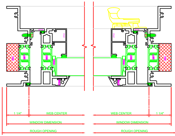
443 JAMB SERIES: 450G CASEMENT OUT 4-BAR ARMS
